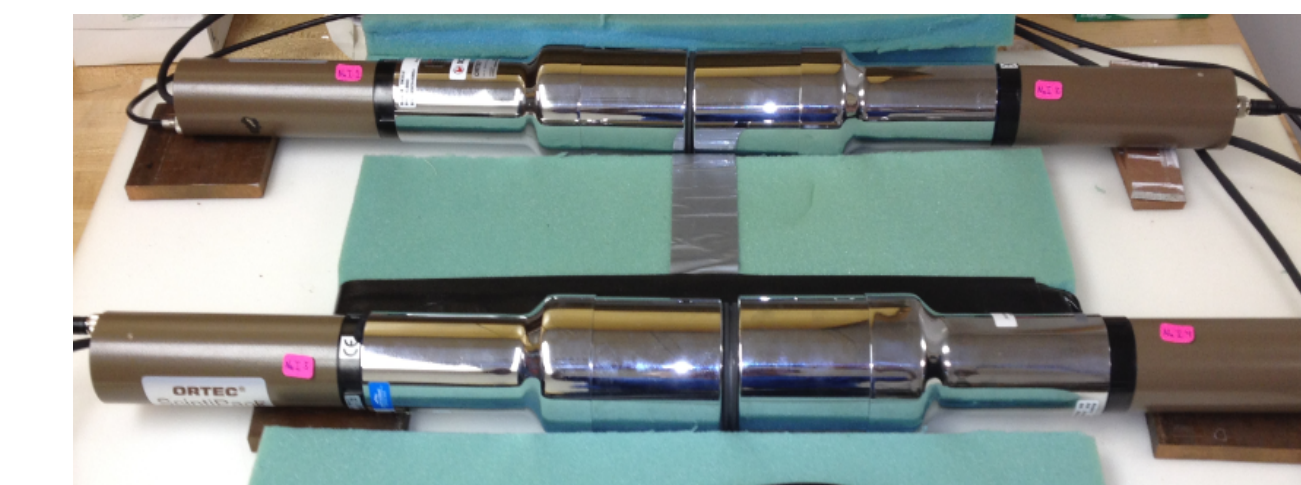
Two pairs of 3 inch by 3 inch NaI detectors were used for coincidence counting
